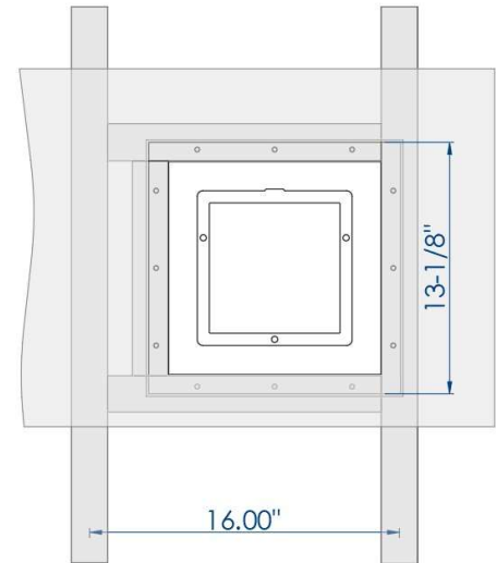
Suggested Drywall Opening
